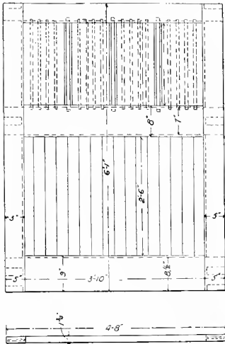
Fig. 1237-1238. Side-doors (2).
